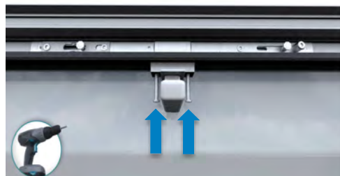
2 Griff verschrauben Fix handle with screws
